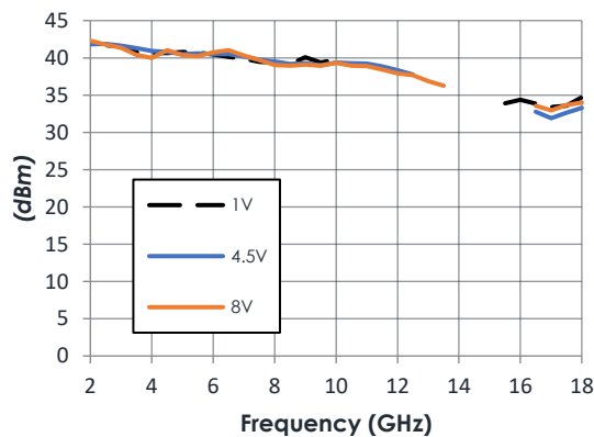
Band 5 Input IP3 vs Bias Voltage
