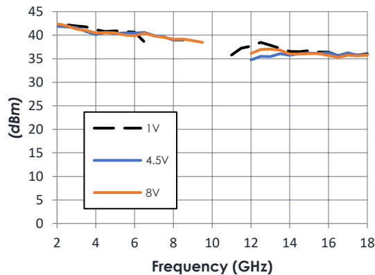
Band 3 Input IP3 vs Bias Voltage
