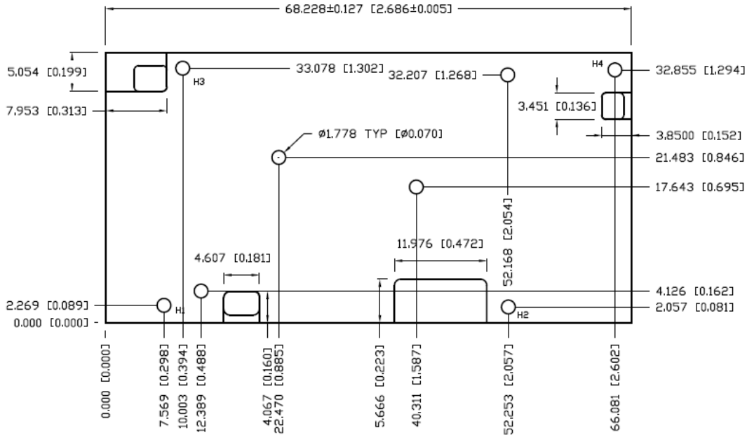
Bottom View
